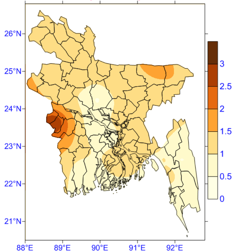
Figure: Spatial distribution of the minimum temperature deviation (in °C) in Bangladesh in 2019
