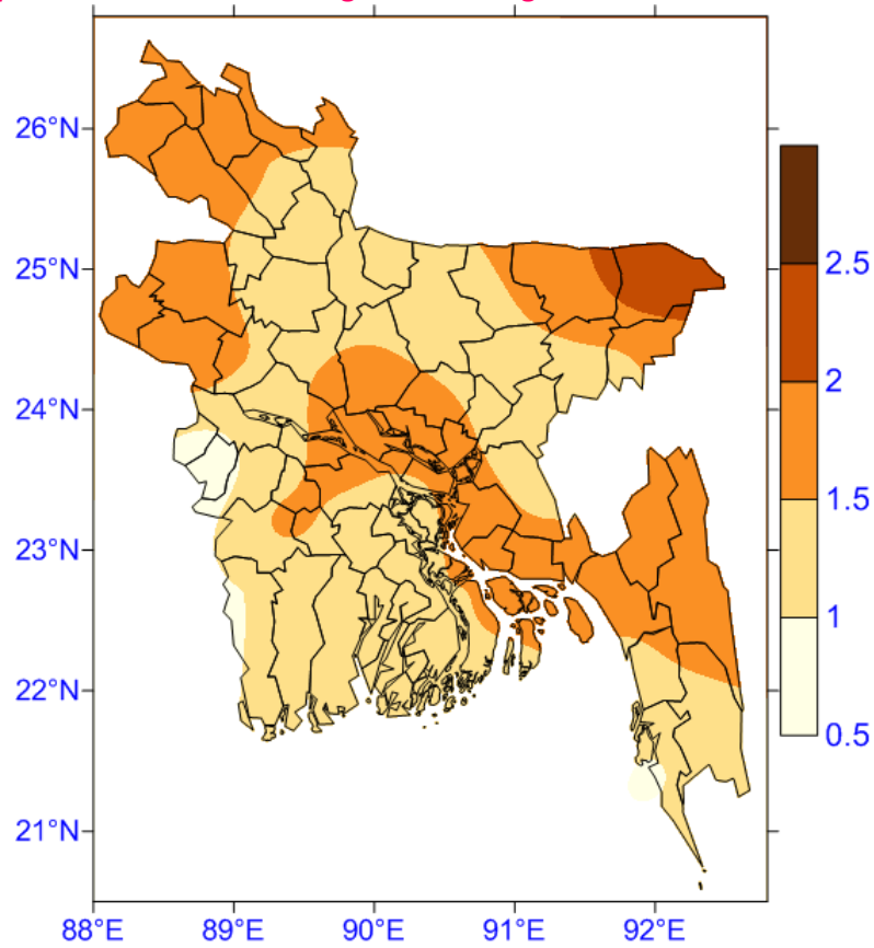
Figure: Spatial distribution of the maximum temperature deviation (in °C) in Bangladesh in 2019
